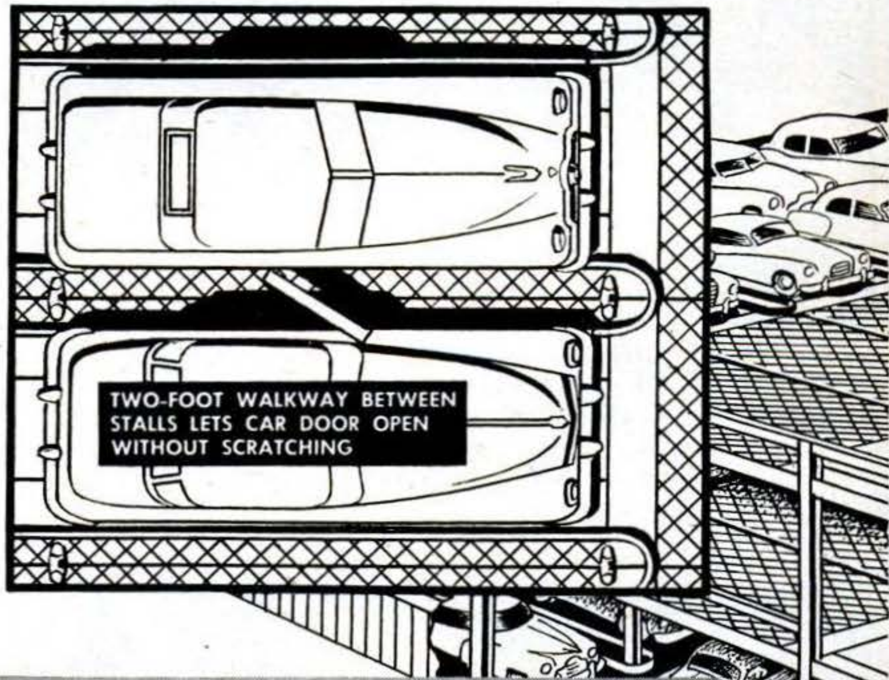
CARS ARE "FUNNELED" into narrow trackways of ramps and parking stalls by converging curbs. Rollers let wheels slip sideways.
